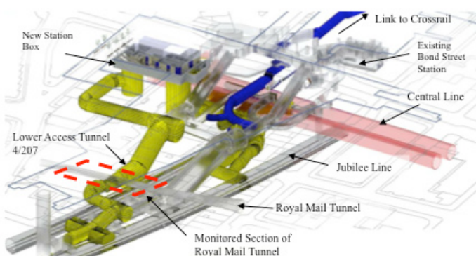
Figure 1: Underground three dimensional view of Bond Street station upgrade scope of works
